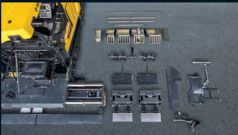
Maximum flexibility: few parts, quickly assembled
